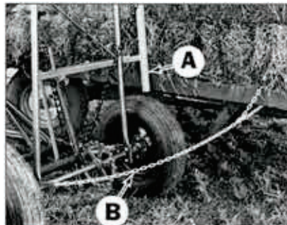
Skid bar (A) maintains correct position of loader against bed. Hillside chain (B) is standard equipment. (Used only on steep hillsides and with wagon.)
