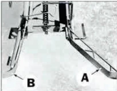
Left pick-up arm (A) is generally used to align bales. If necessary, right pick-up arm may also be used to align bales. Clevis guard (B) is removed for towing.
